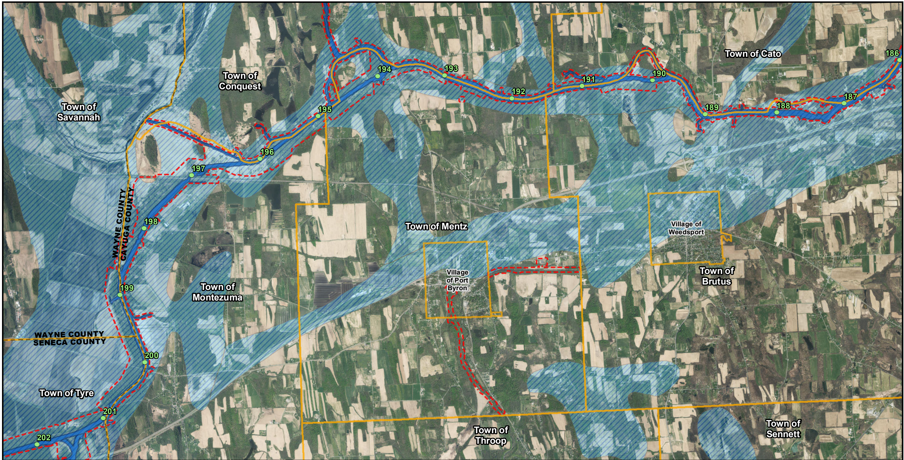
Figure 82F: Aquifers
